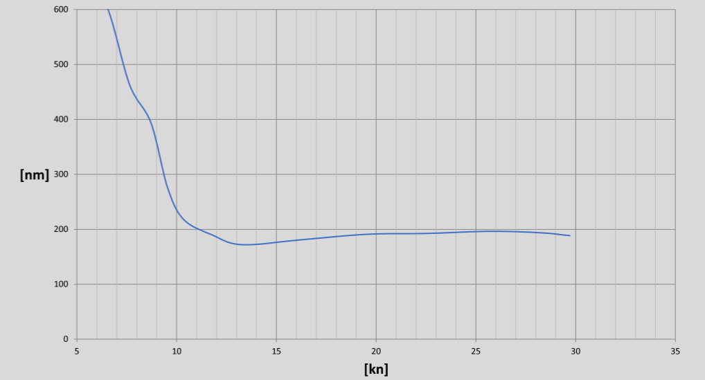
"F500" - "Cummins 550hp" Range in nm
