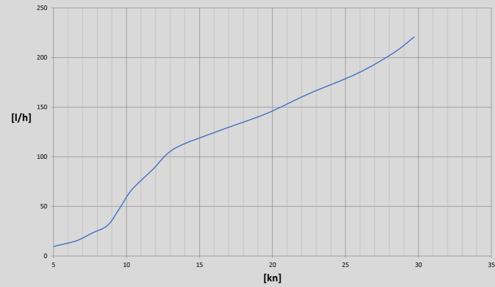
"F500" - "Cummins 550hp" Fuel consumption [l/h]
