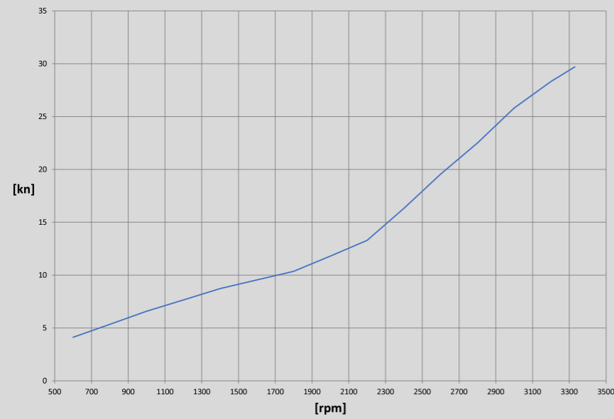
"F500" - "Cummins 550hp" Speed [kn]
