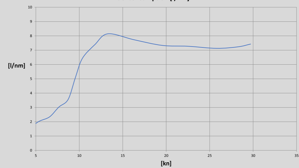
"F500" - "Cummins 550hp" Fuel consumption [l/nm]
